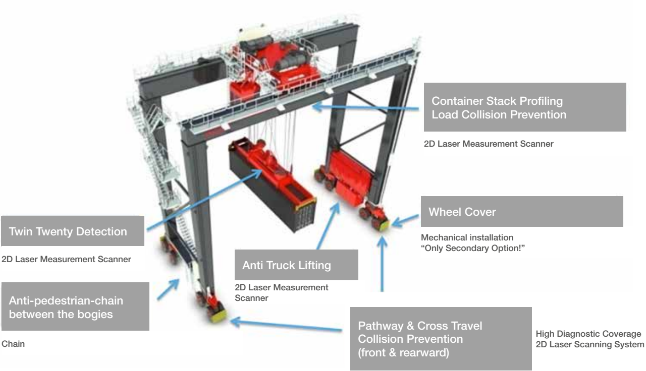
Figure: Collision Prevention Solutions at RTG
