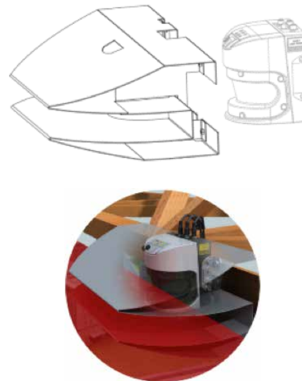
Figure: Weatherhood
