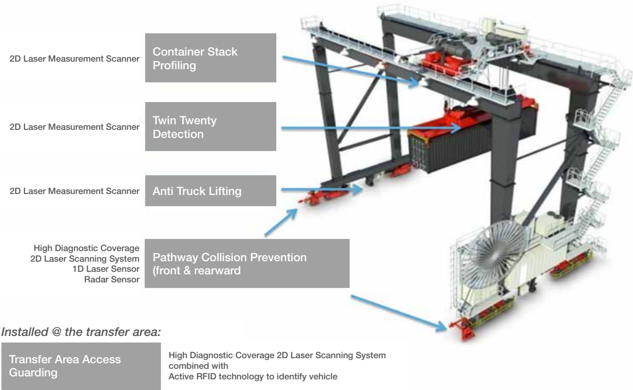
Figure: Collision Prevention Solutions for ASCs
